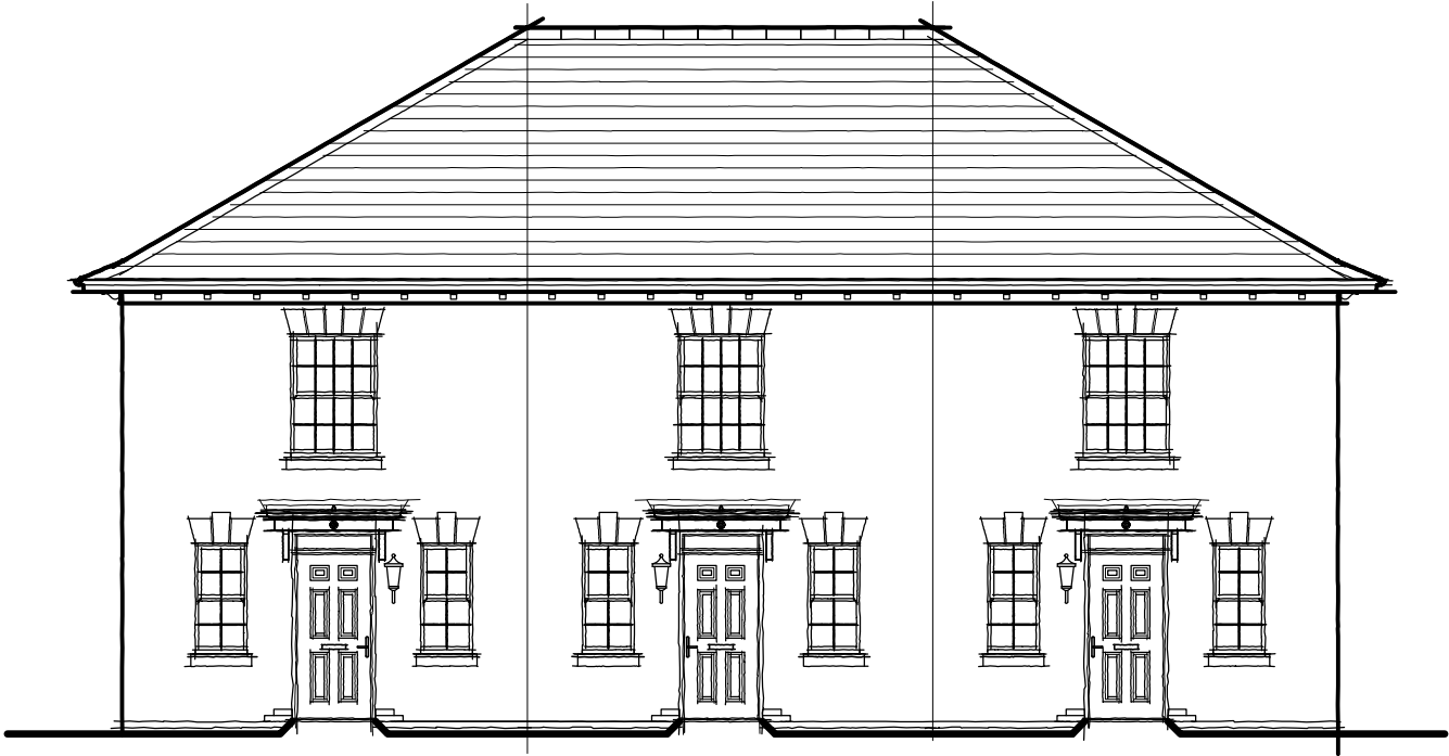
Rear Elevations
