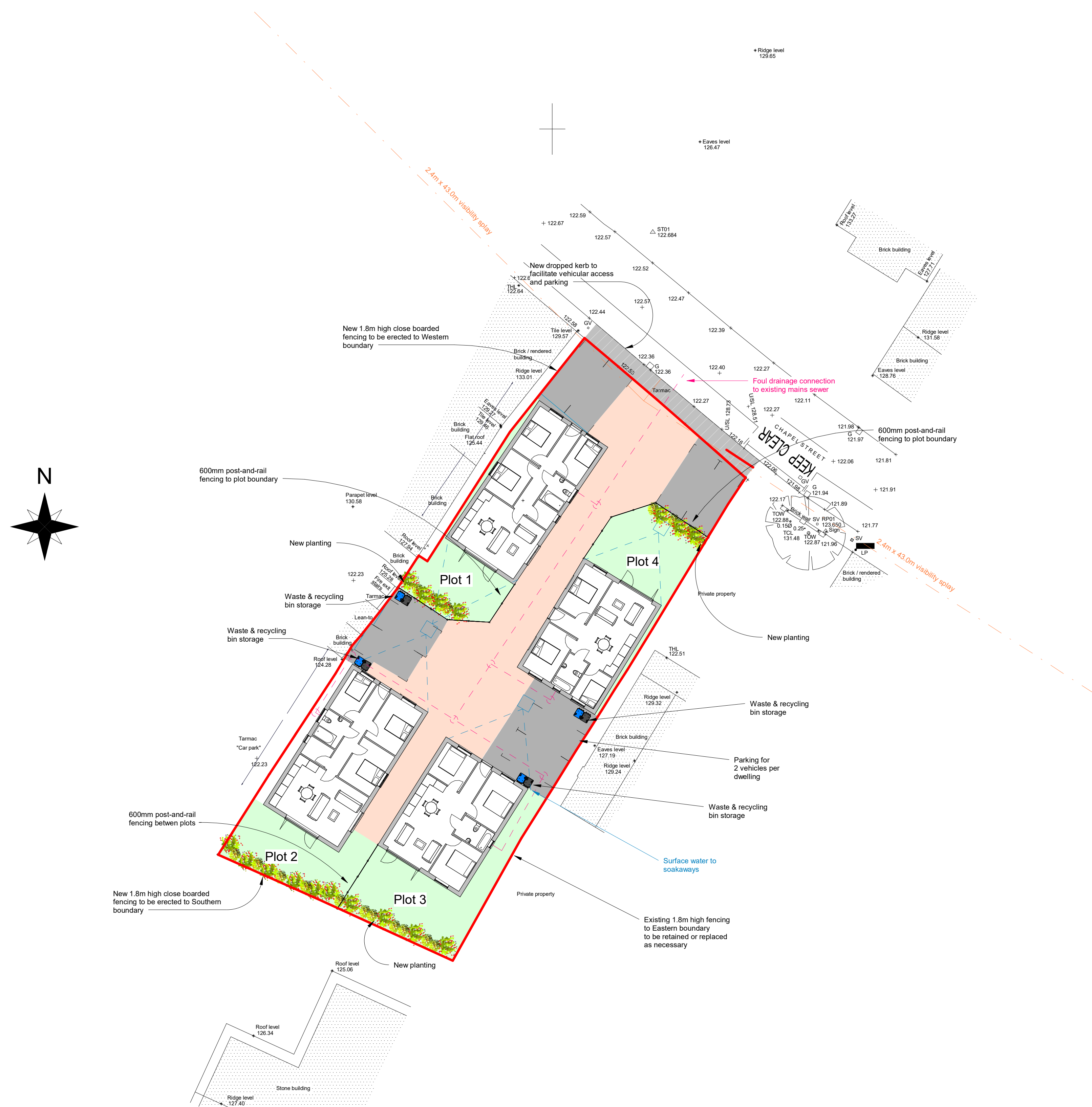
1 Proposed Block Plan
