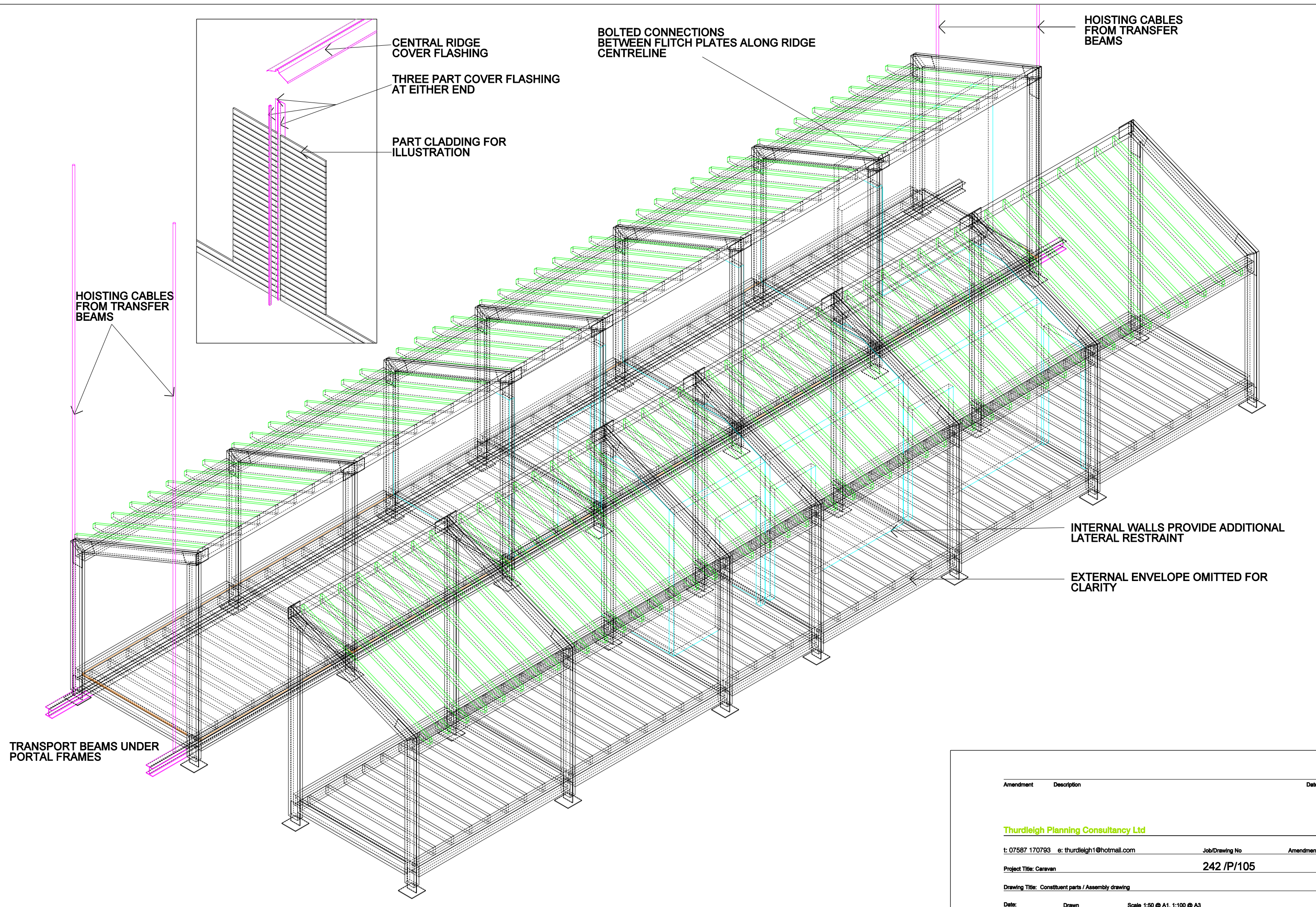
OVERALL 3D VIEW NTS
