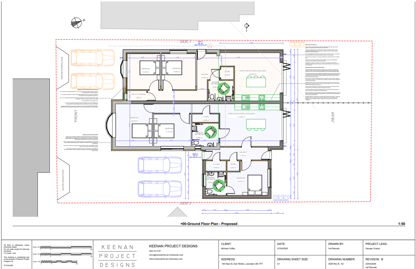
Fig.3. Proposed plans.
