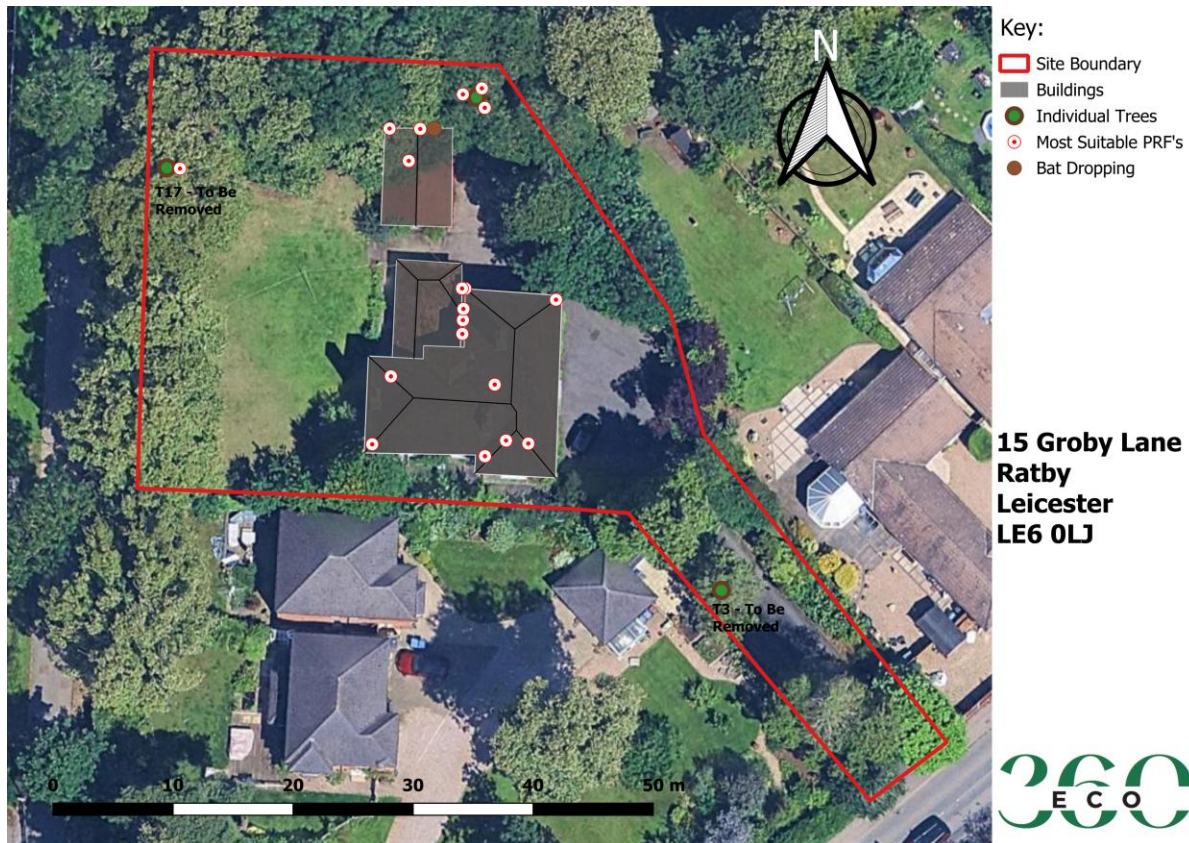
Fig.3. Feature map
