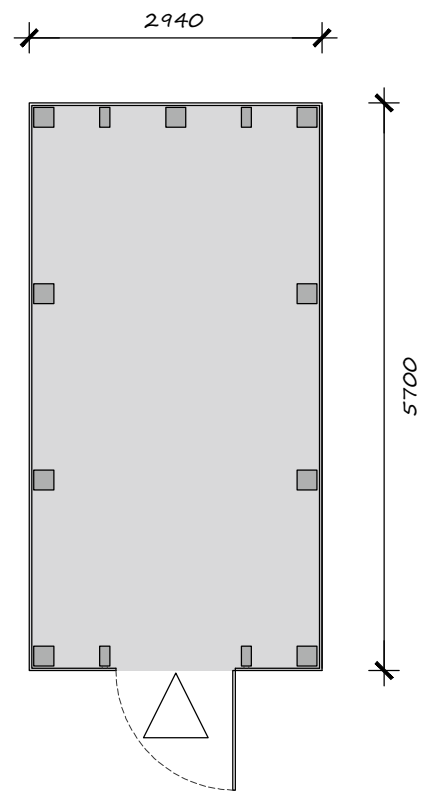
Floor Plan
