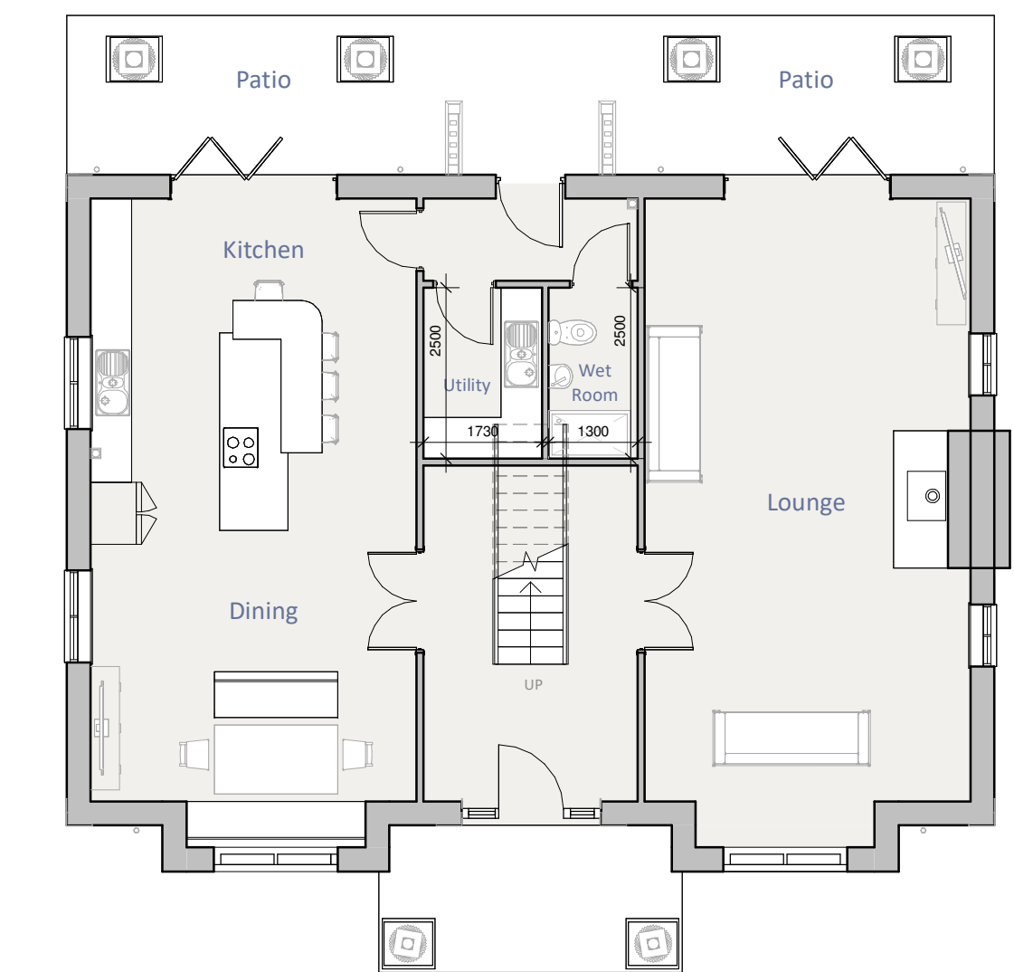
Ground Floor
