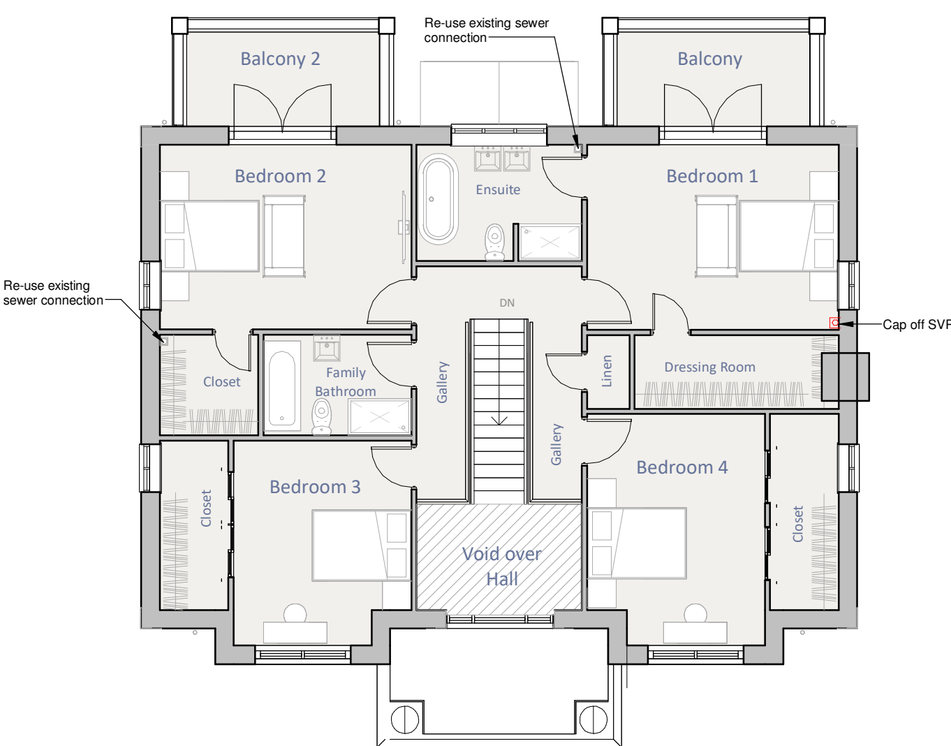
First Floor
