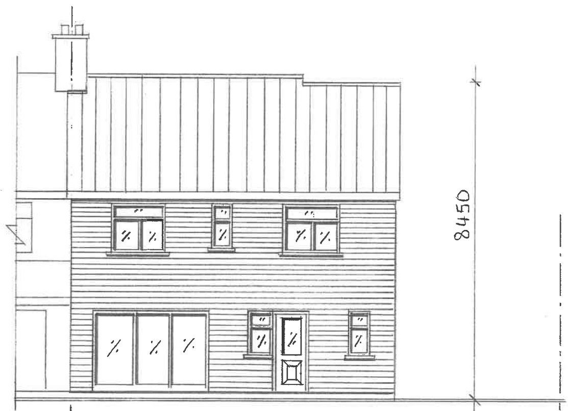
PROPOSED REAR ELEVATION - N
