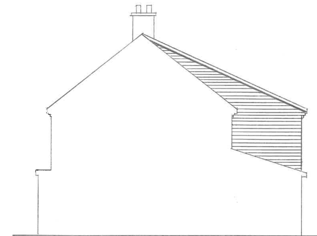
PROPOSED SIDE ELEVATION - E
