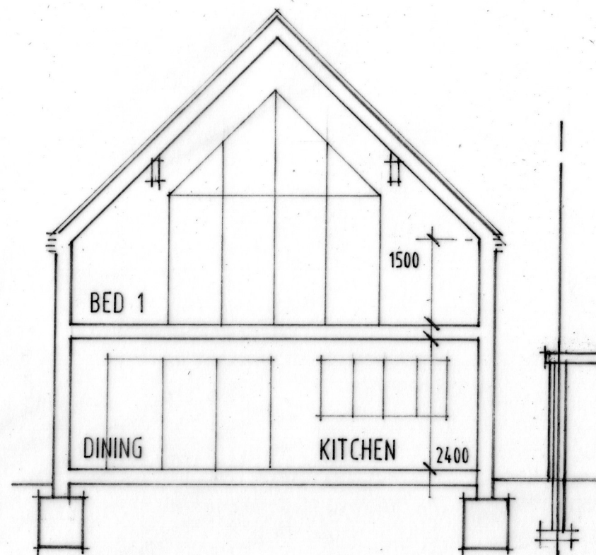
SECTION B
