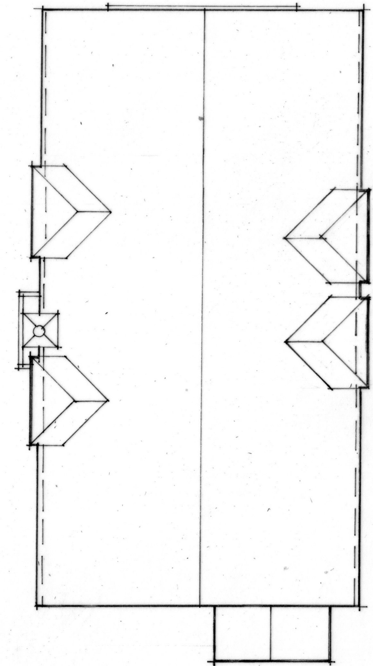
ROOF PLAN
