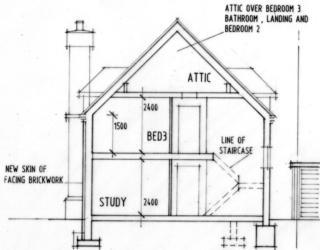
SECTION A
