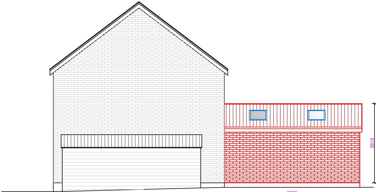
NORTH-WEST ELEVATION
