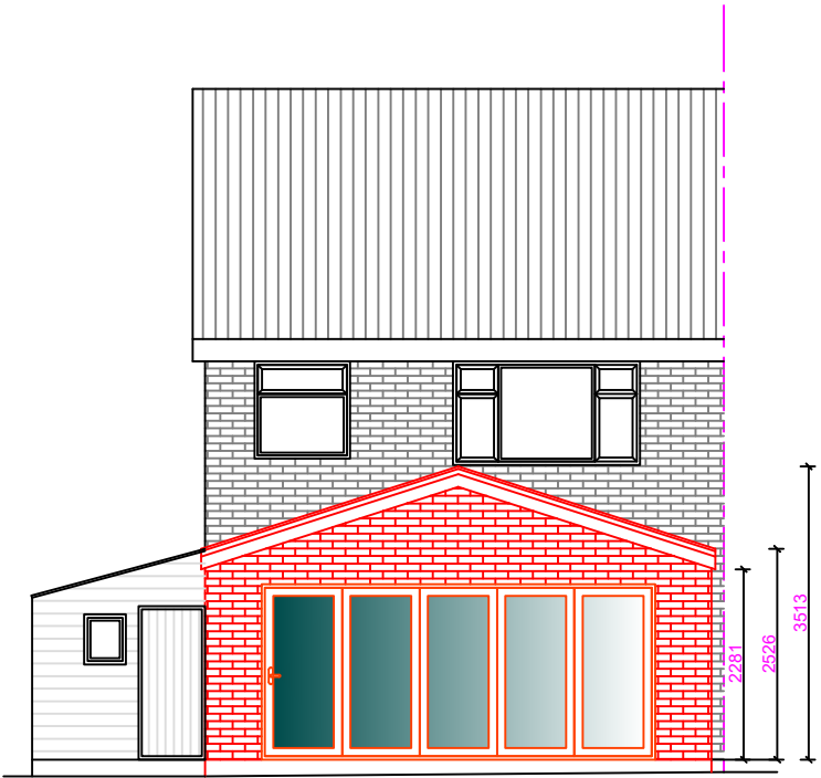
SOUTH-WEST ELEVATION
