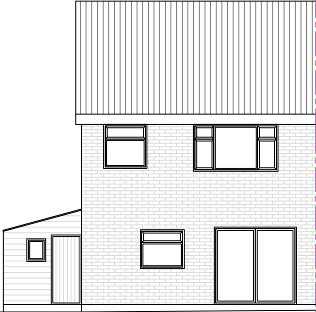
SOUTH-WEST ELEVATION
