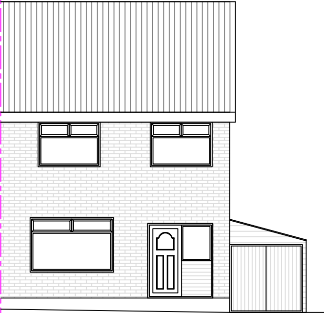
NORTH-EAST ELEVATION
