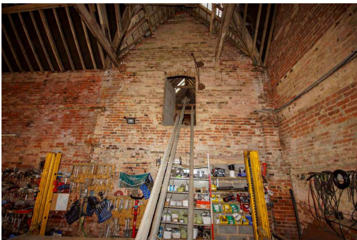
Plate 62: G2 – gable with taking-in door and adjacent iron bracket of former hoist
