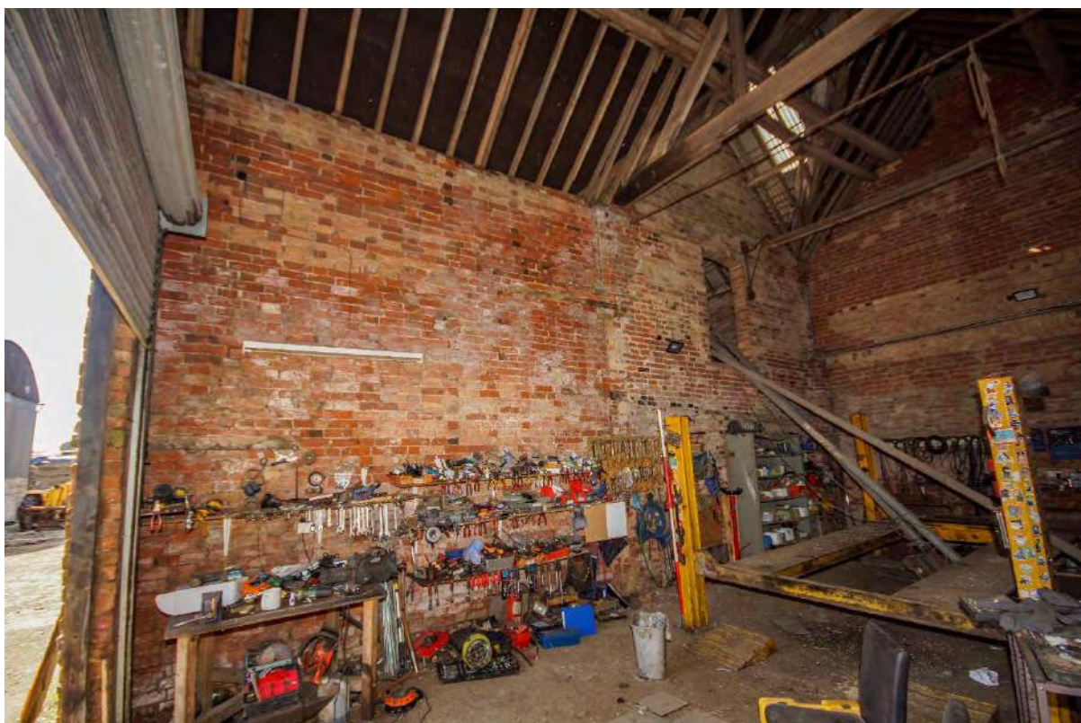
Plate 61: G2 – southeast wall with construction joint to the gable wall
