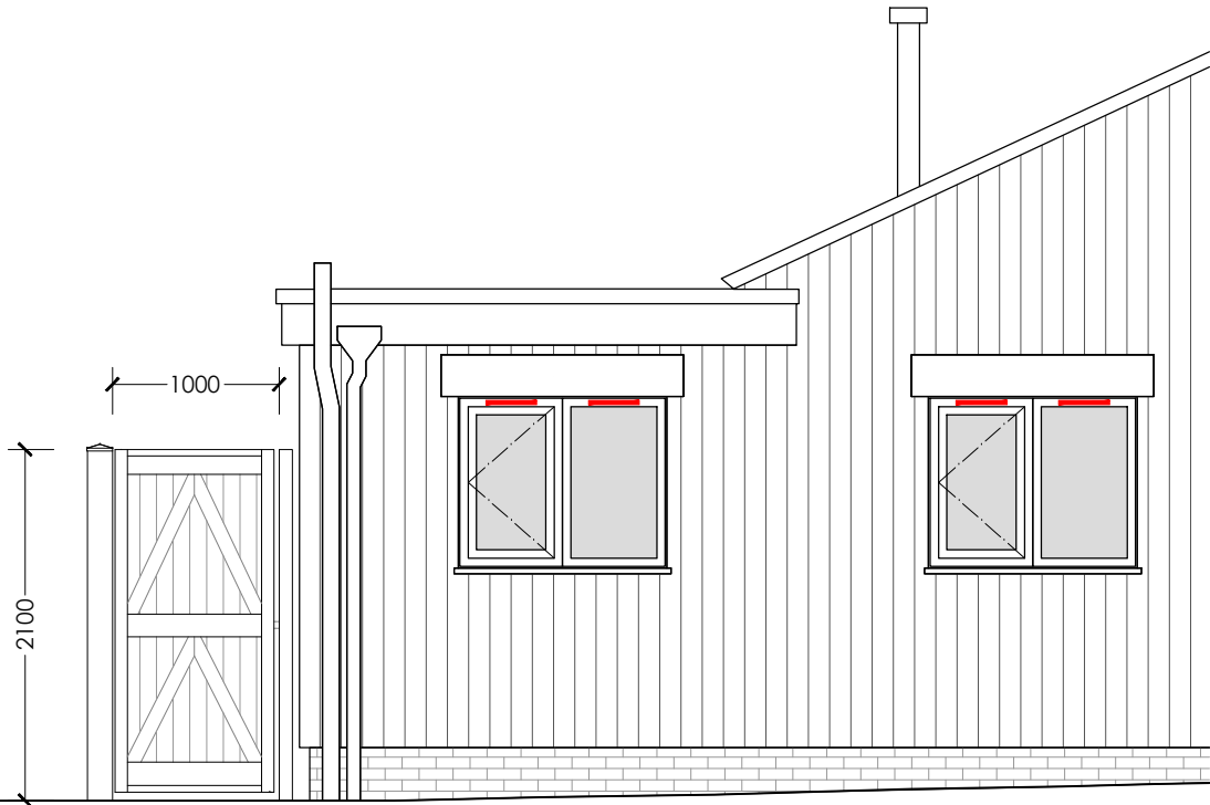
Proposed wooden security gate, 2.1 x 1.0m Existing fencing retained.
