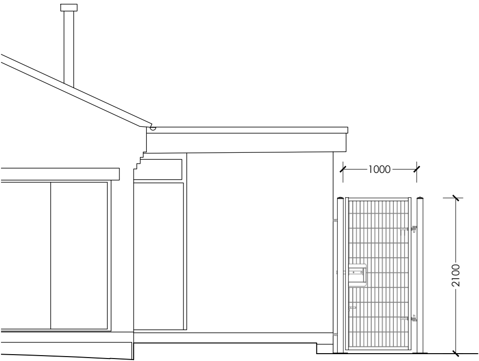
Existing side (west) part-elevation
