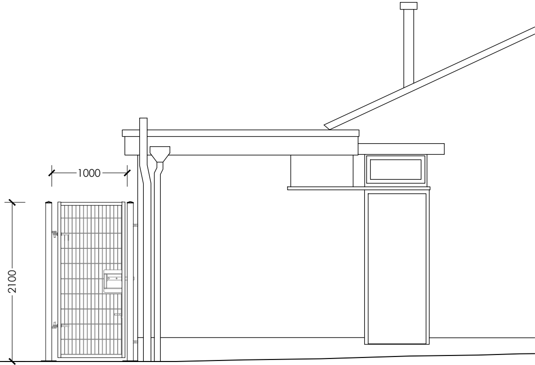
Existing single leaf mesh security gate, galvanised and powder coated green. 2.1 x 1.0m
