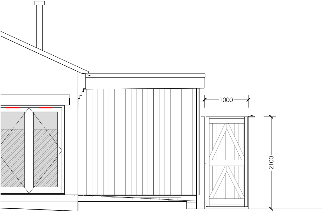
Proposed side (west) part-elevation
