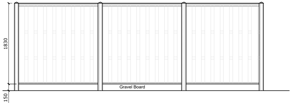
Hit and Miss Fence Enclosure Scale 1:50
