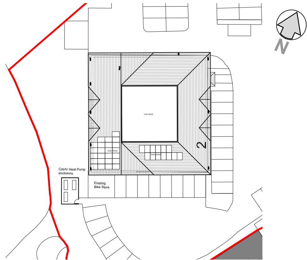
CAHV Enclosure Location on Site Scale 1:500
