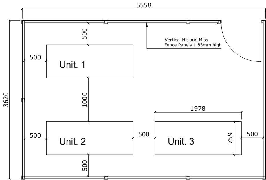
CAHV Heat Pump enclosure Scale 1:50
