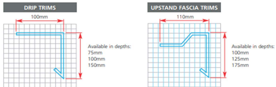
Figure 12: Polyroof Edge Trim profiles, compatible with flat roofing
