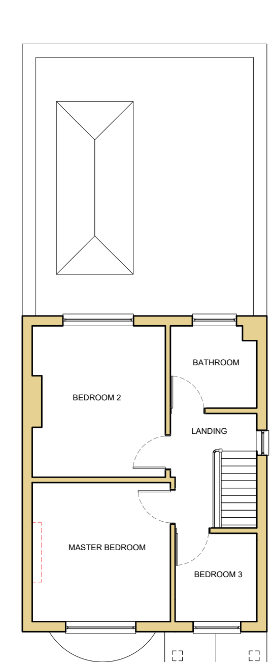
PROPOSED FIRST FLOOR/ ROOF PLAN 1:100
