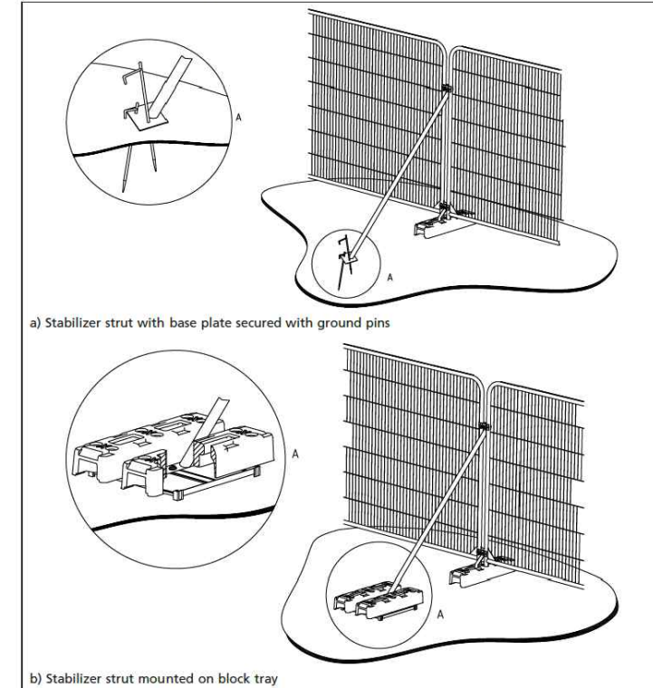
Figure 3 Examples of above-ground stabilizing systems
