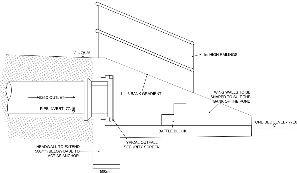
SECTION VIEW
