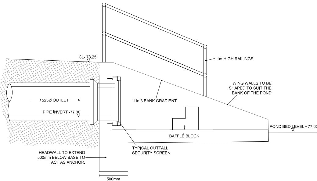
SECTION VIEW
