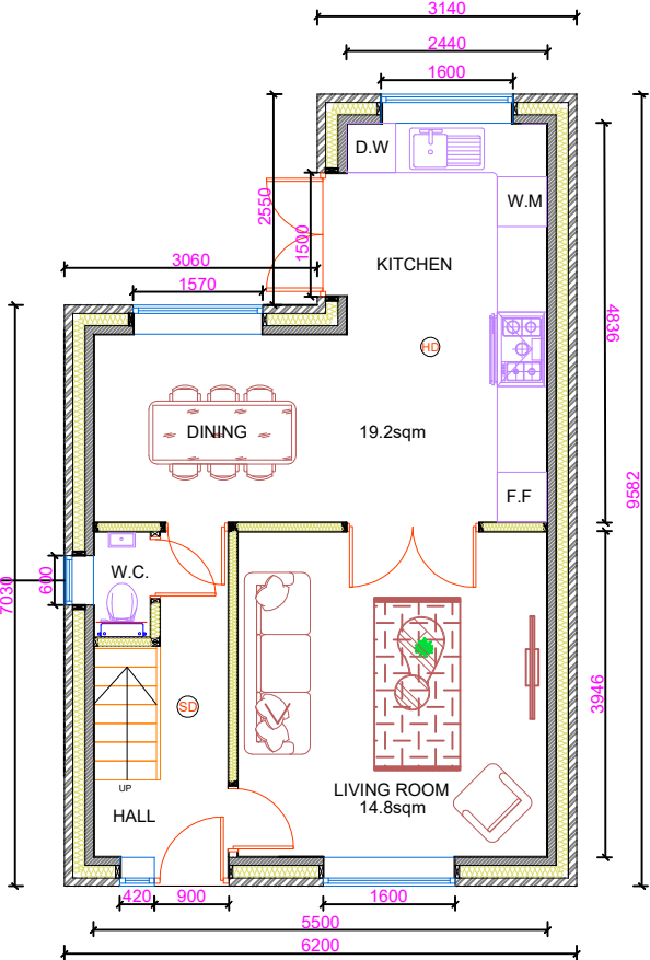
Proposed Ground Floor Plan @ 1:100 (A3)
