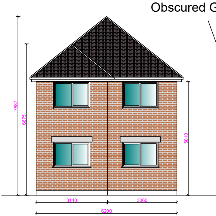
Proposed Rear Elevation (South West) @ 1:100 (A3)
