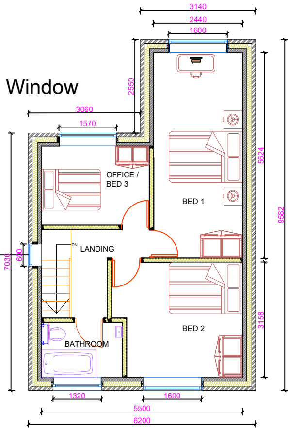
Proposed First Floor Plan @ 1:100 (A3)
