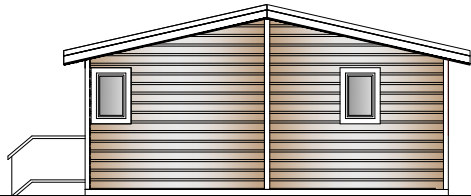
Rear Elevation
