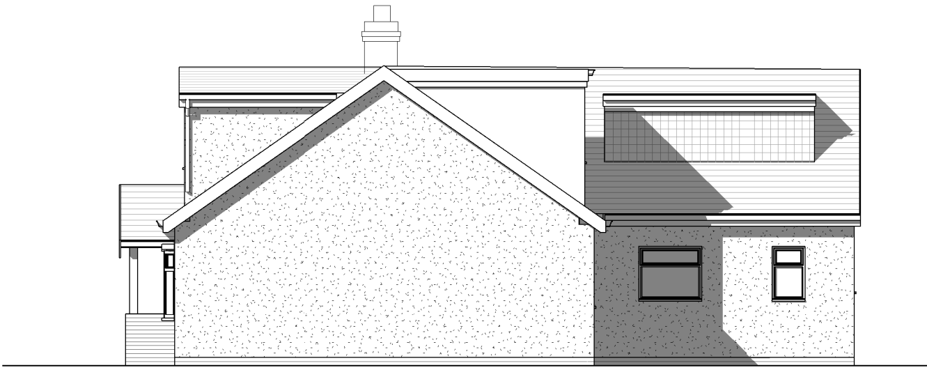
Side Elevation
