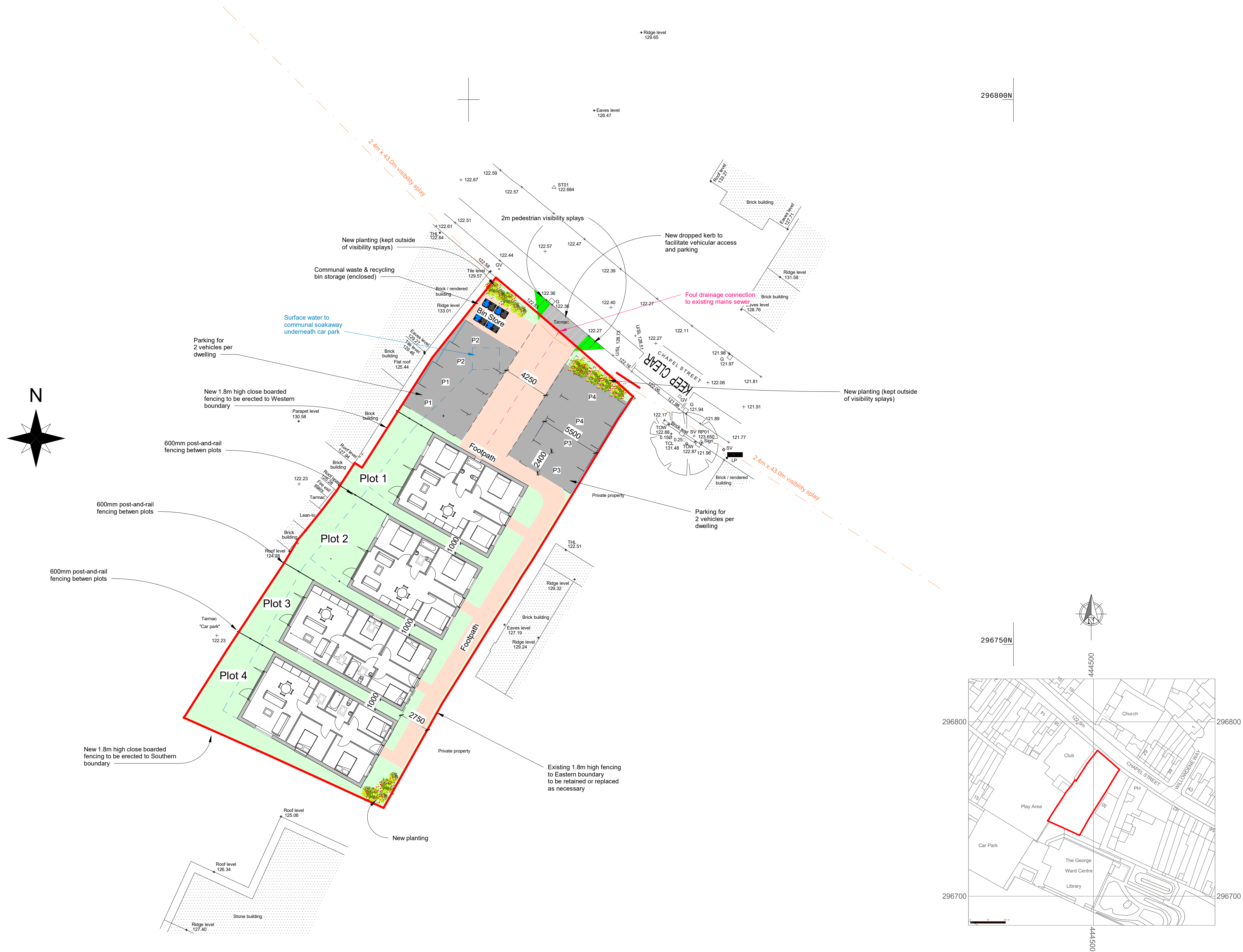
1 Proposed Block Plan 1 : 200
