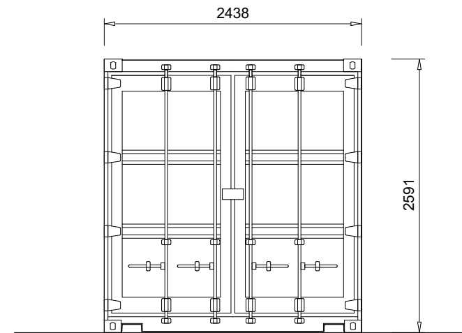
02 FRONT ELEVATION 1:50
