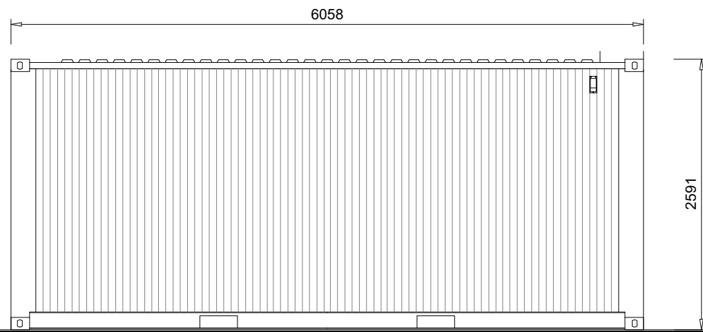
03 SIDE ELEVATIONS 1:50
