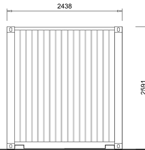
04 REAR ELEVATION 1:50
