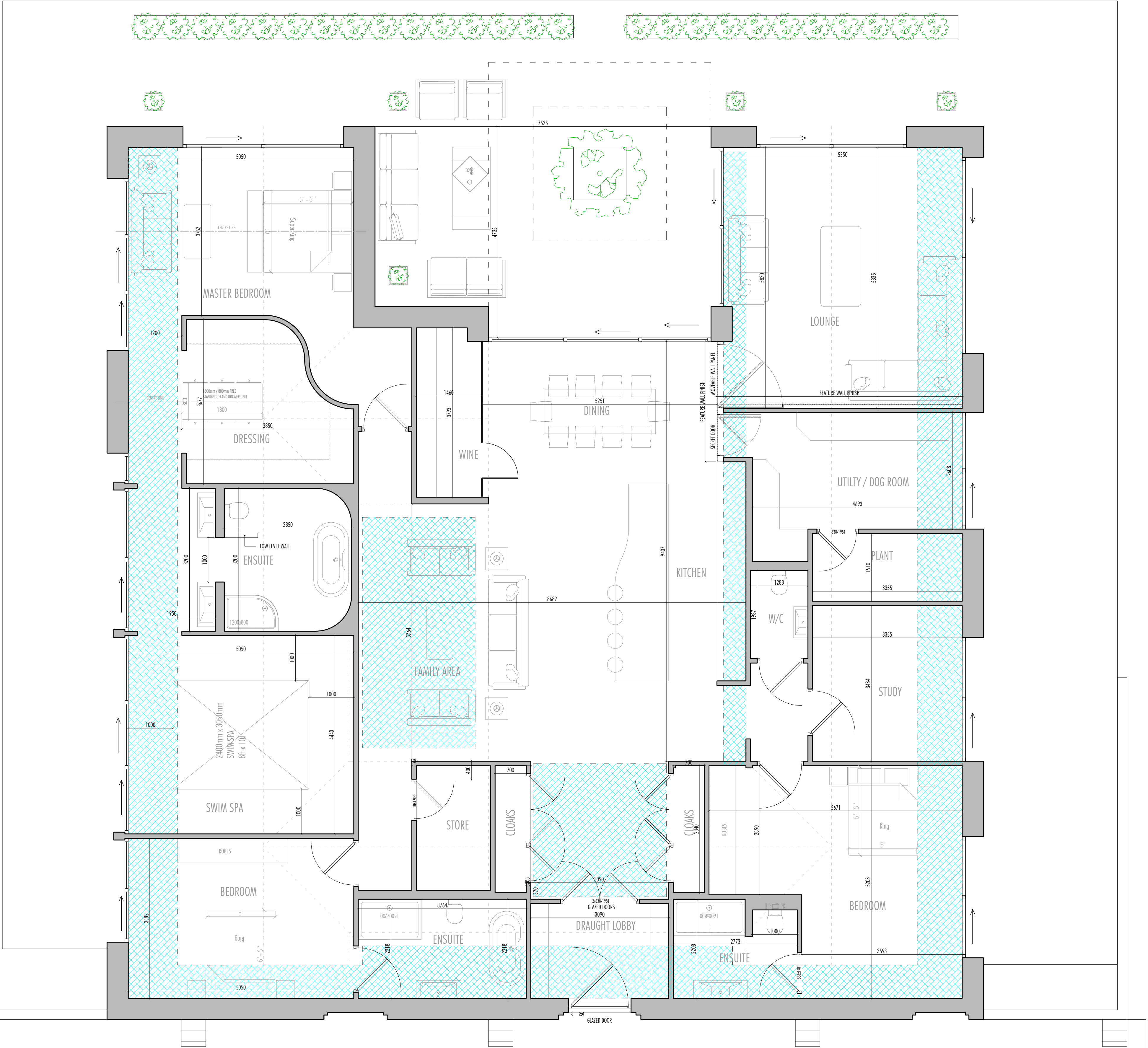
Proposed Plan [1:50]
