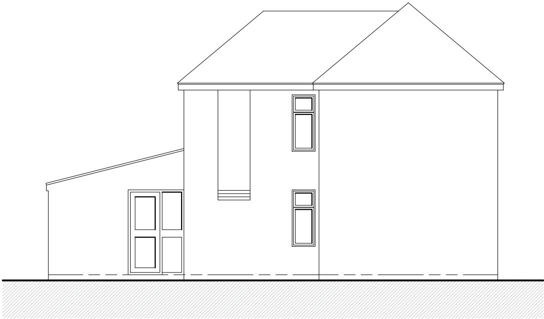
EXISTING WEST SIDE ELEVATION
