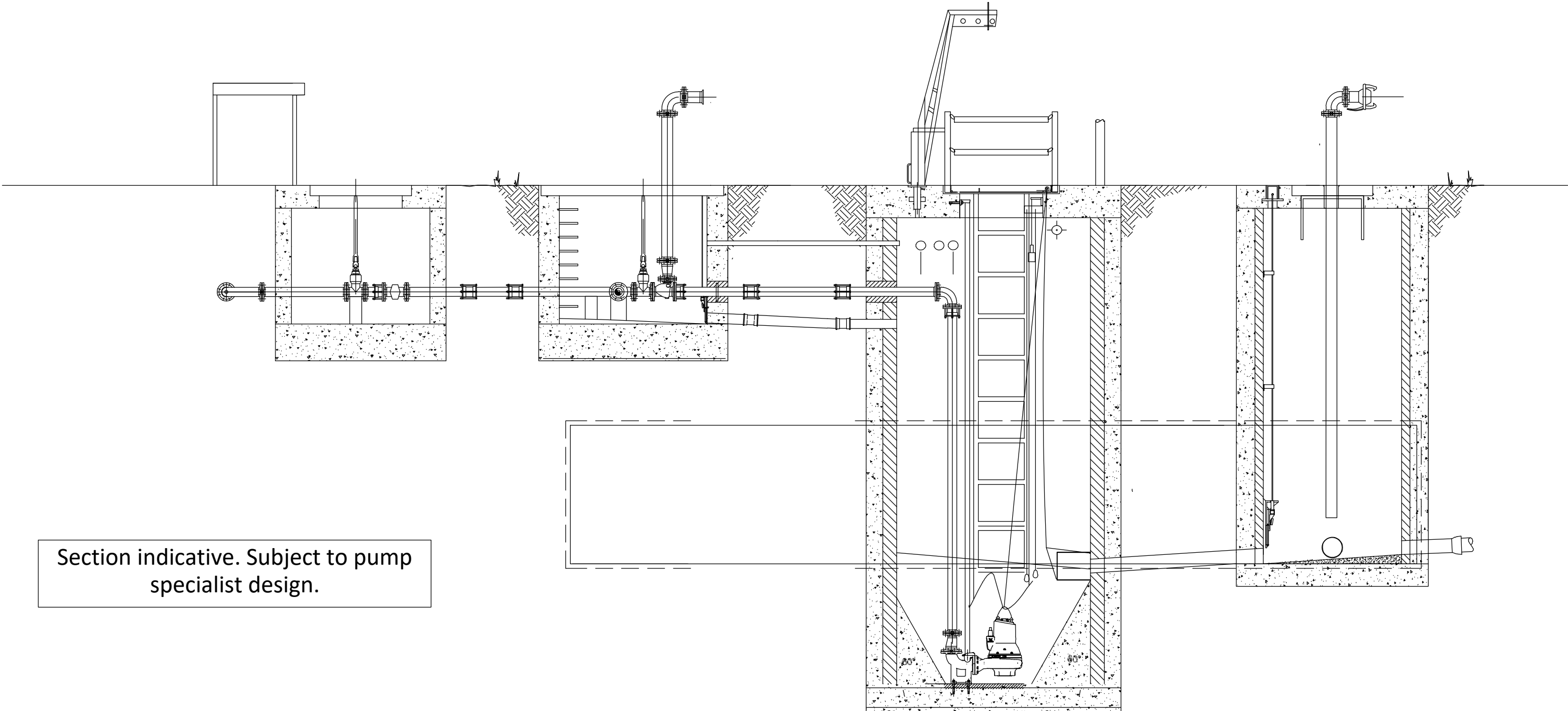
SECTION THROUGH
