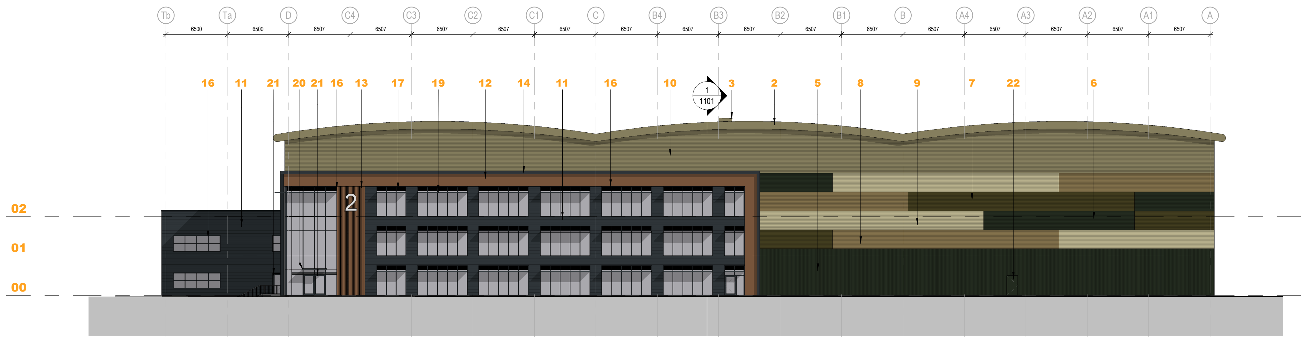
1: GA ELEVATION 1 1 : 250
