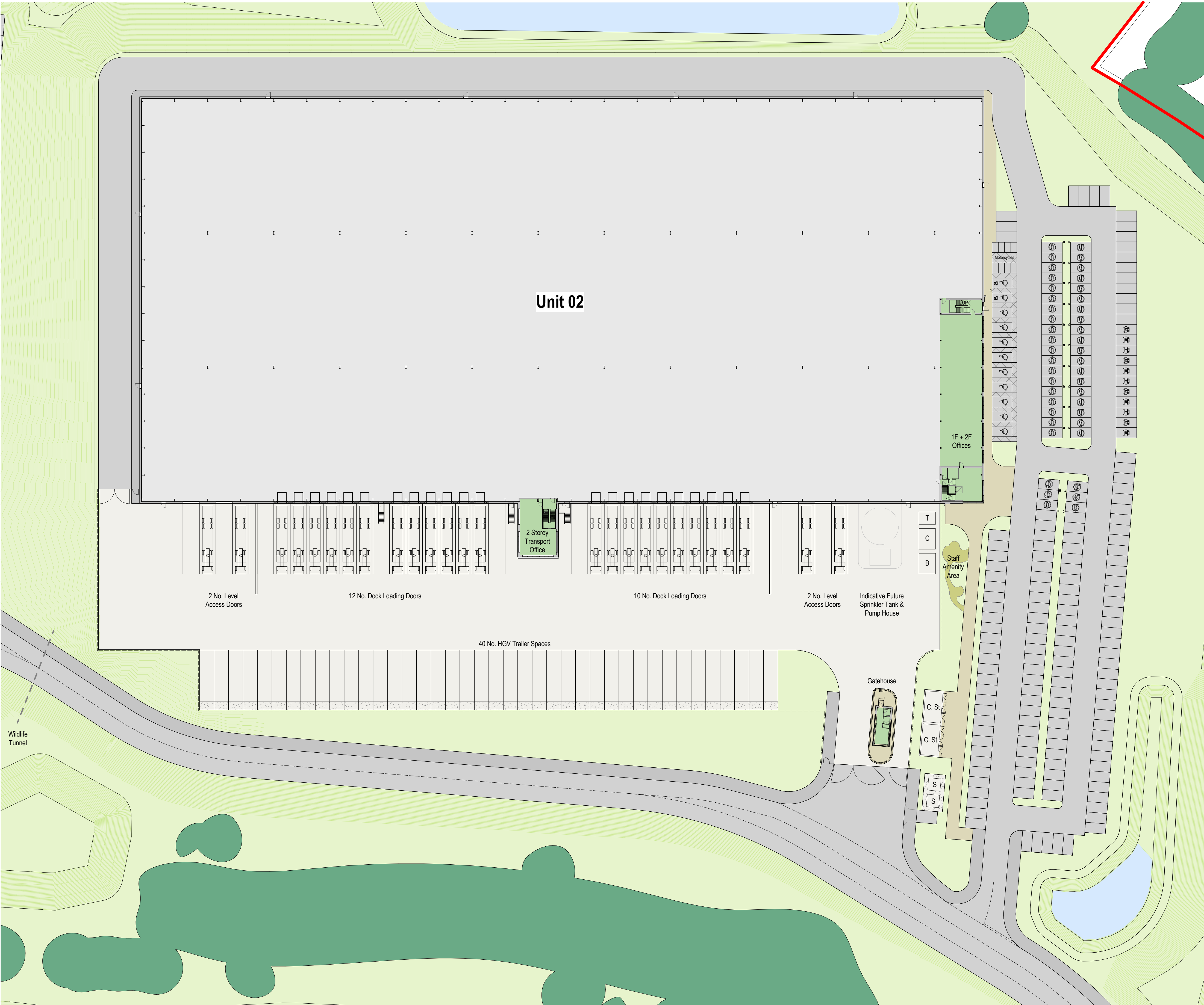
UNIT 02 - PROPOSED SITE PLAN
