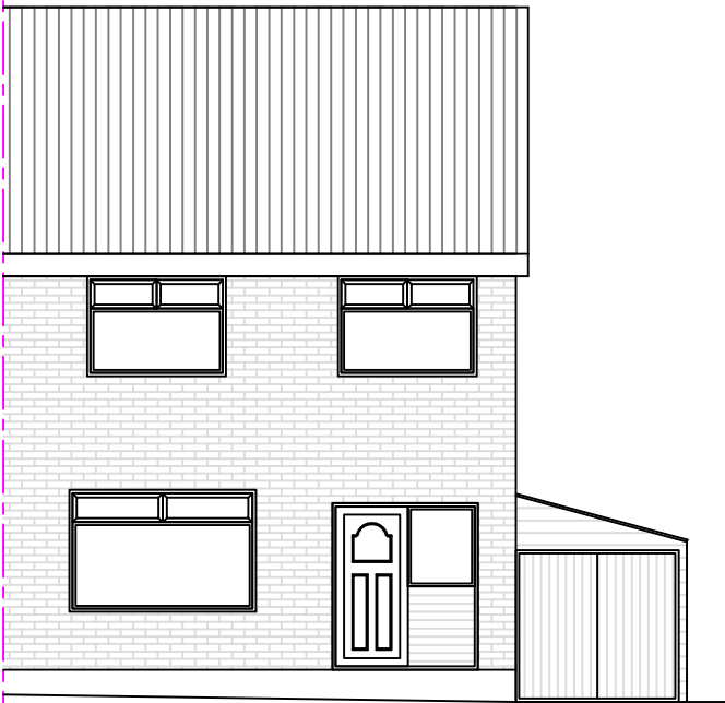
NORTH-EAST ELEVATION
