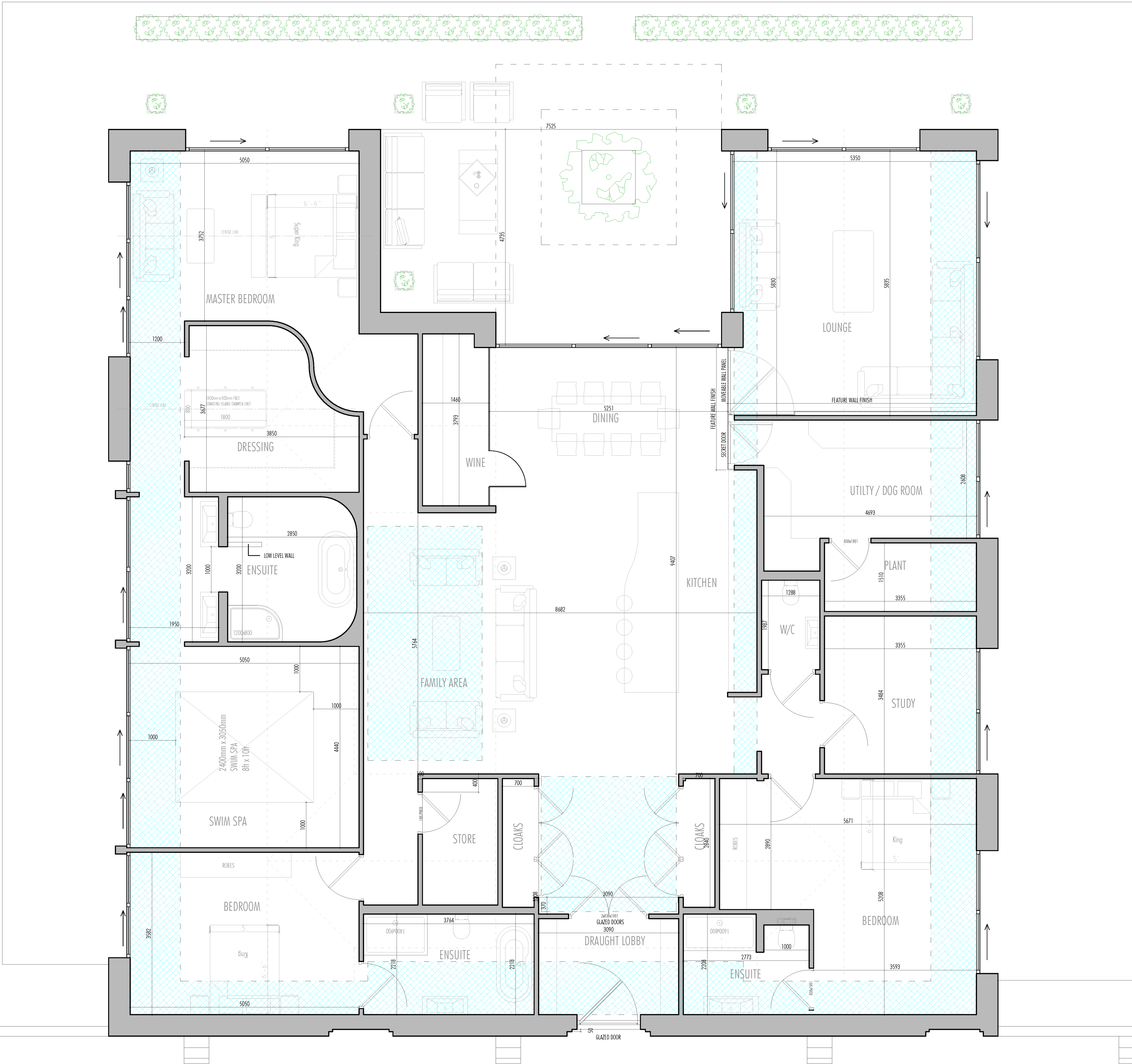
Proposed Plan [1:50]
