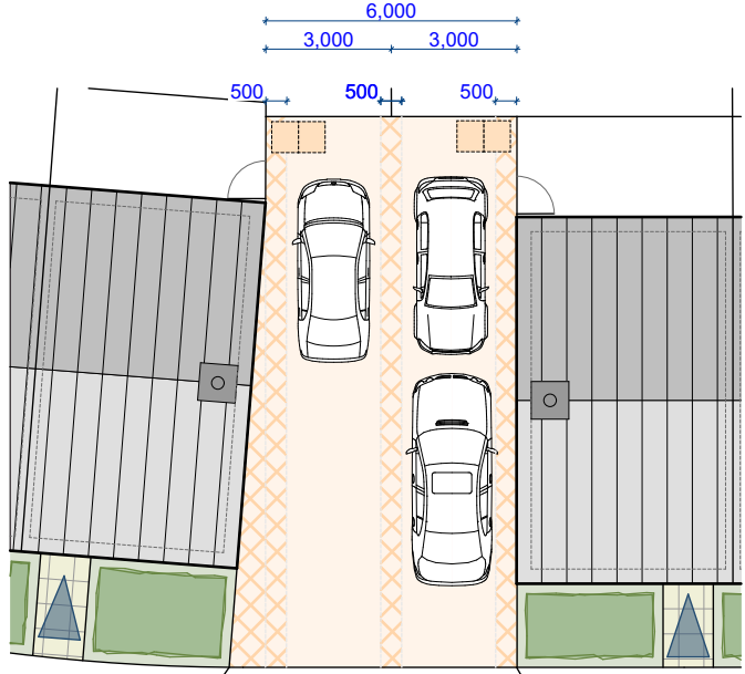
Car Parking Setting Out (Driveway) Scale: 1:200
