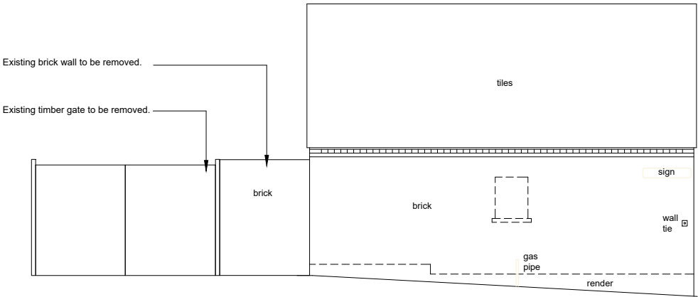
East elevation
