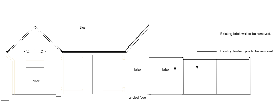
West elevation
