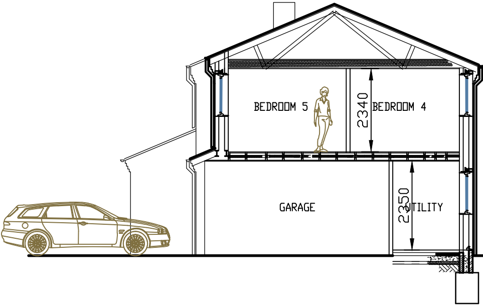
PROPOSED SECTION
