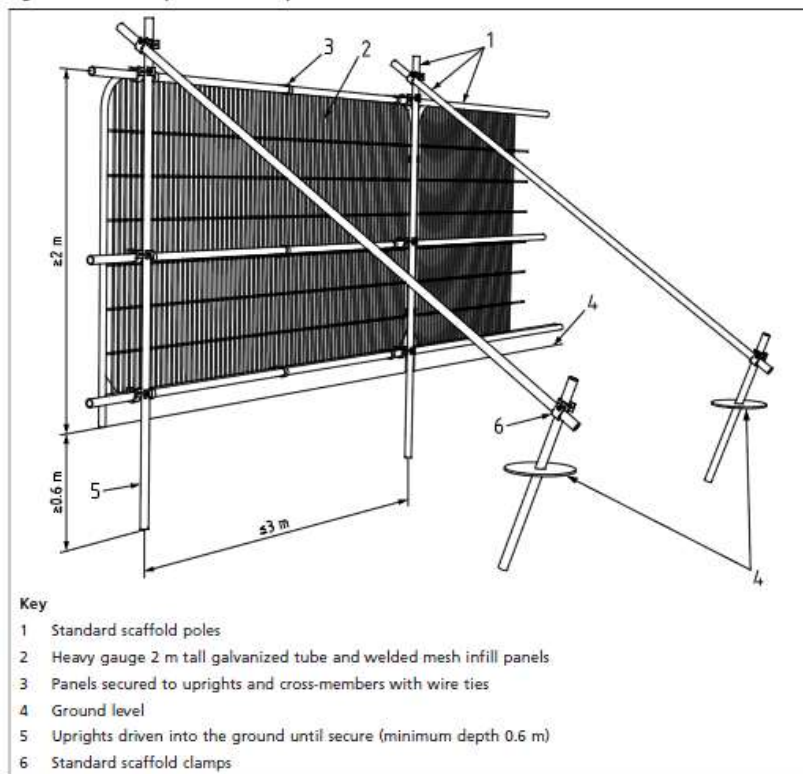
Figure 4 - Tree Protection Barrier
