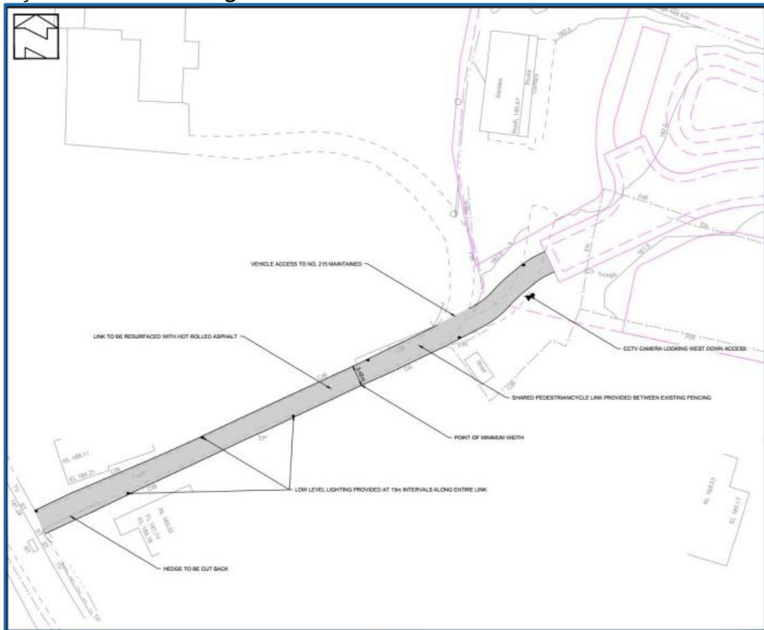
Figure 3: Proposed Development Site layout plan
