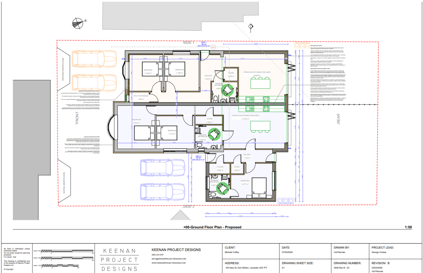
Fig.3. Proposed plans.
