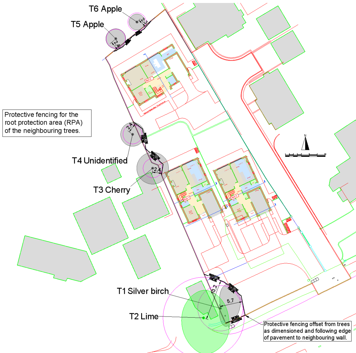
Extract from the tree protection plan showing siting of protective fencing.
