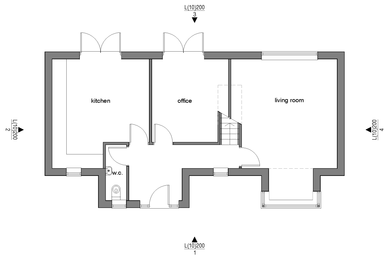
EXISTING PLAN
