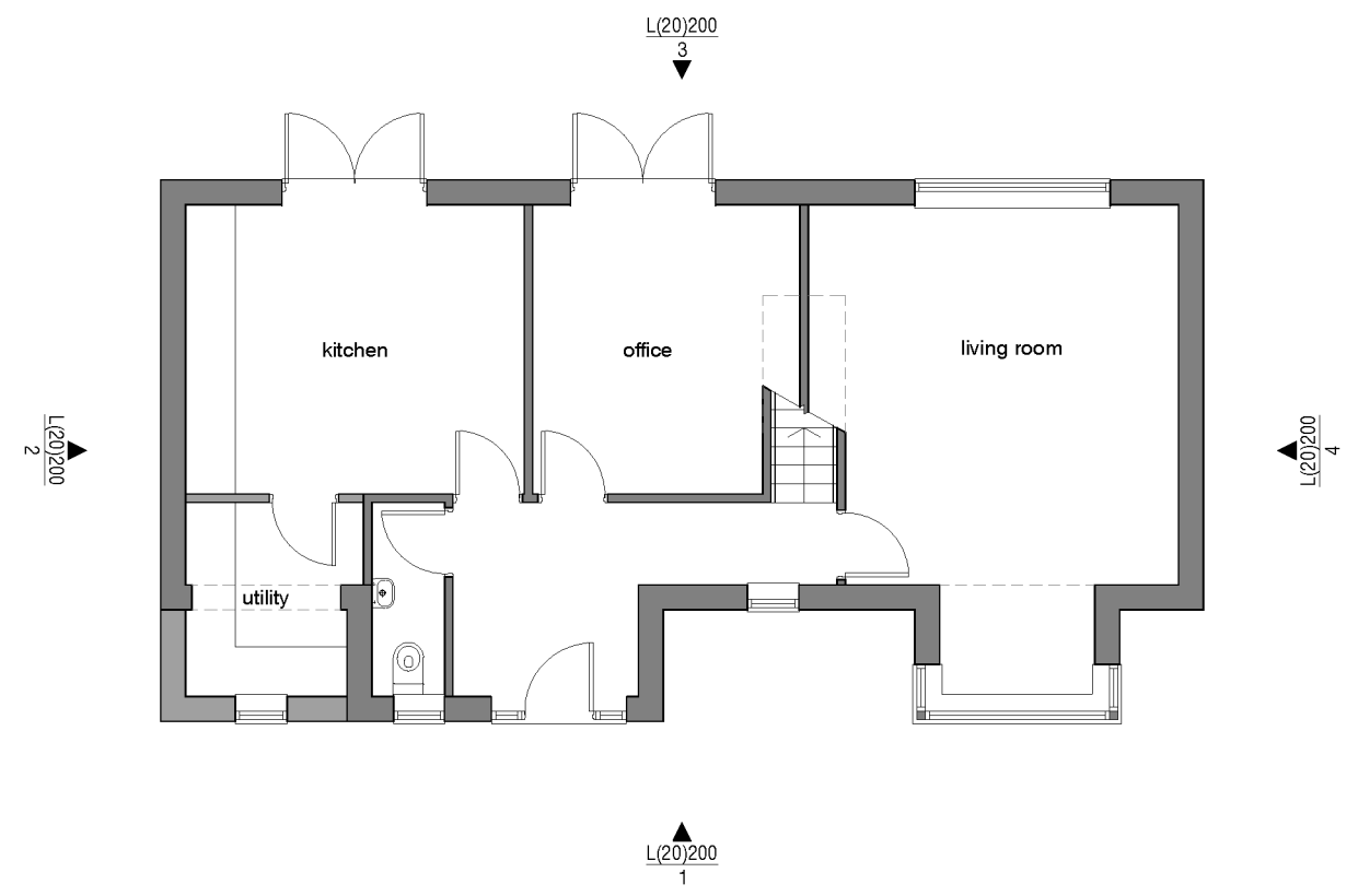
PROPOSED PLAN
