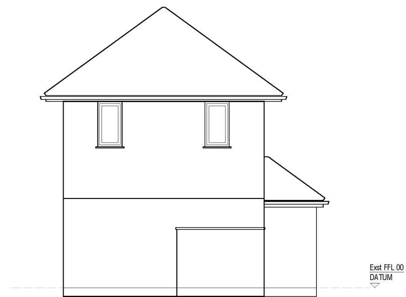
2. EXISTING SIDE ELEVATION
