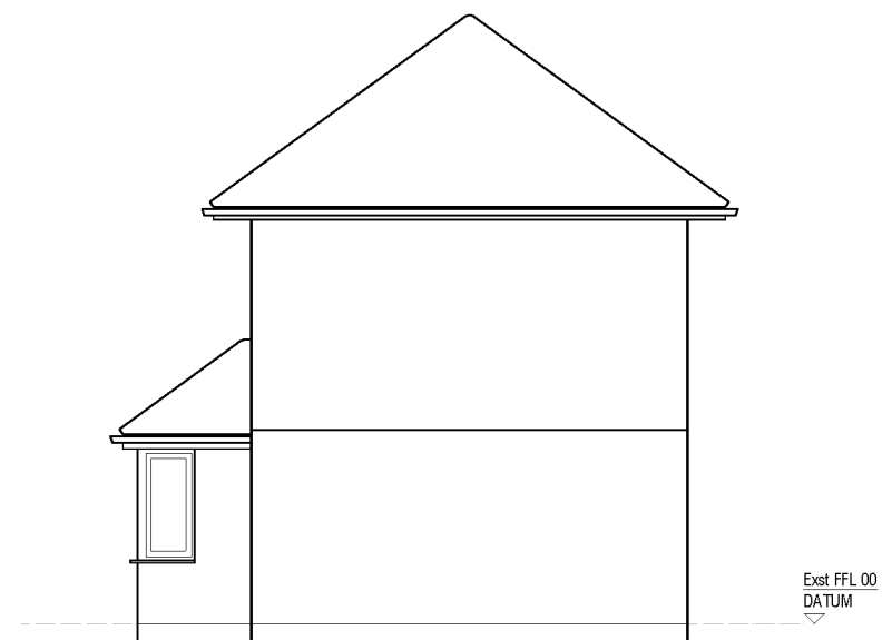
4. EXISTING SIDE ELEVATION
