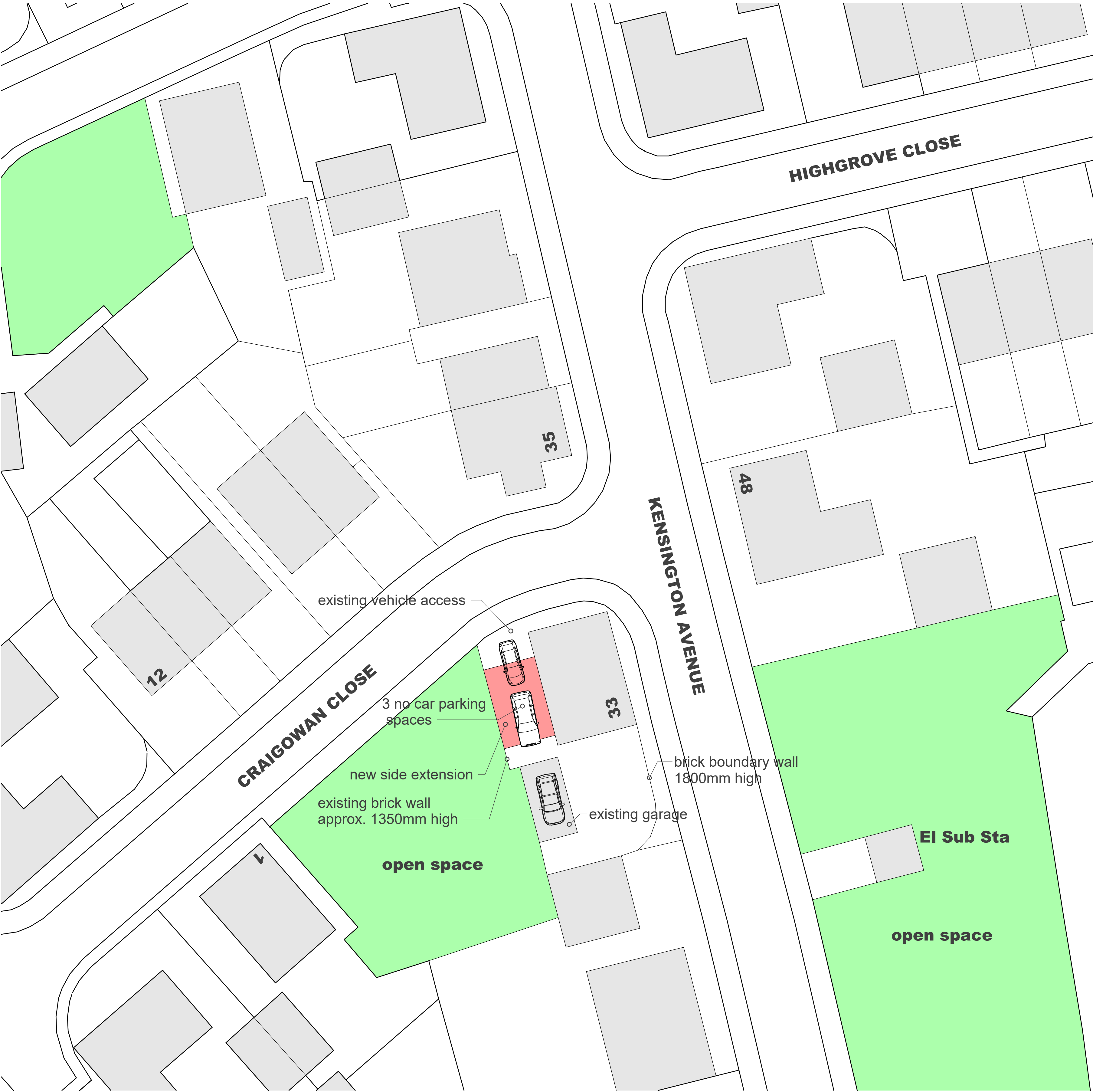
SITE PLAN @ 1:200
