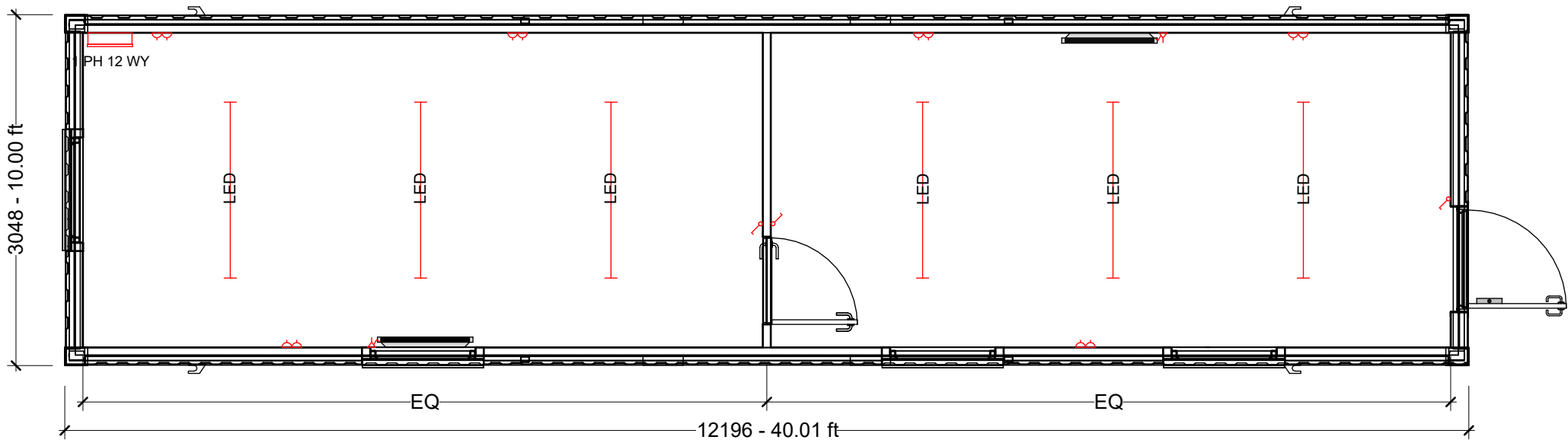
1 General Arrangement 1 : 50
