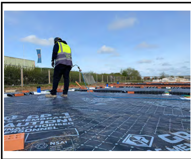
Air lance test on a welded lap.
