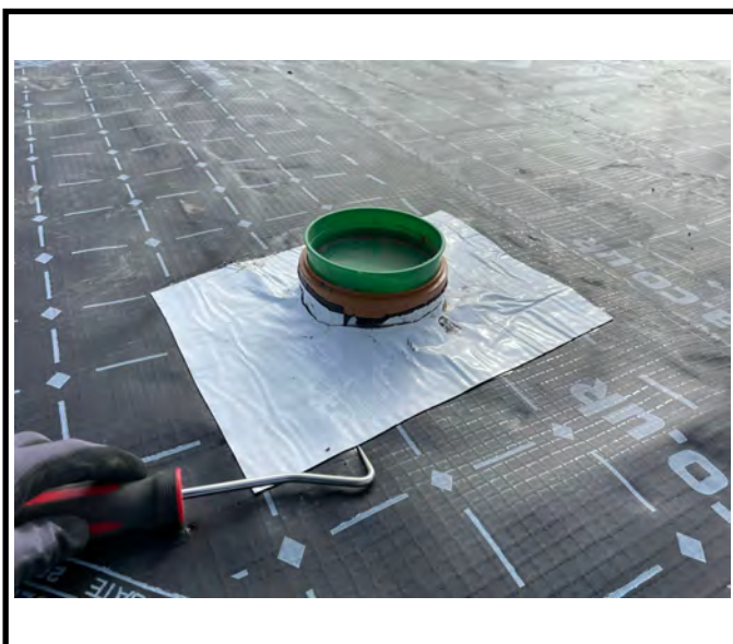
A mechanical point stress test being conducted upon a sealed pipe penetration.
