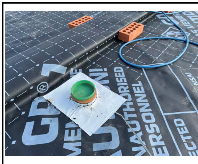
Air lance test on a pipe penetration.
