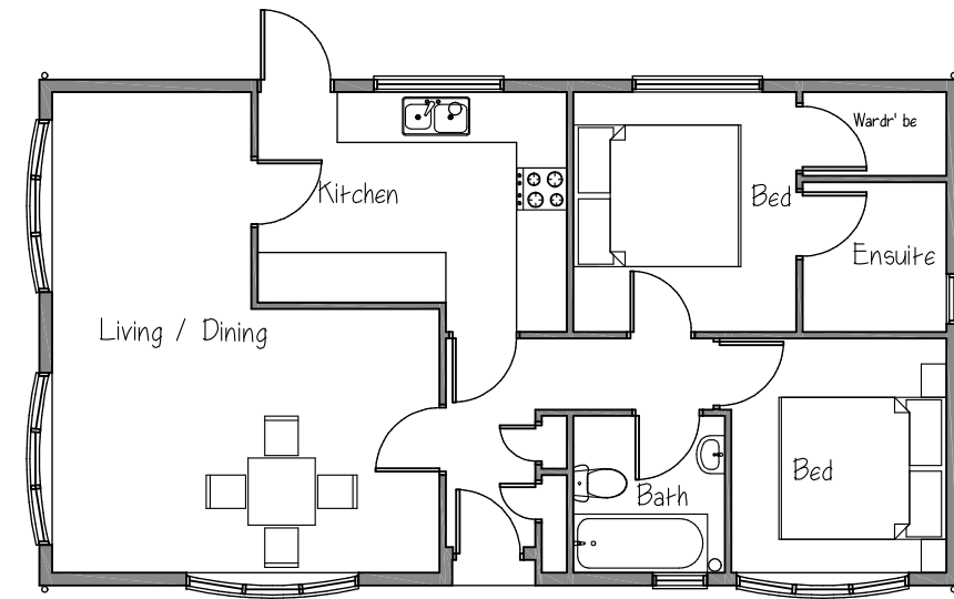
B 2 Bed Park Home Scale 1:100
