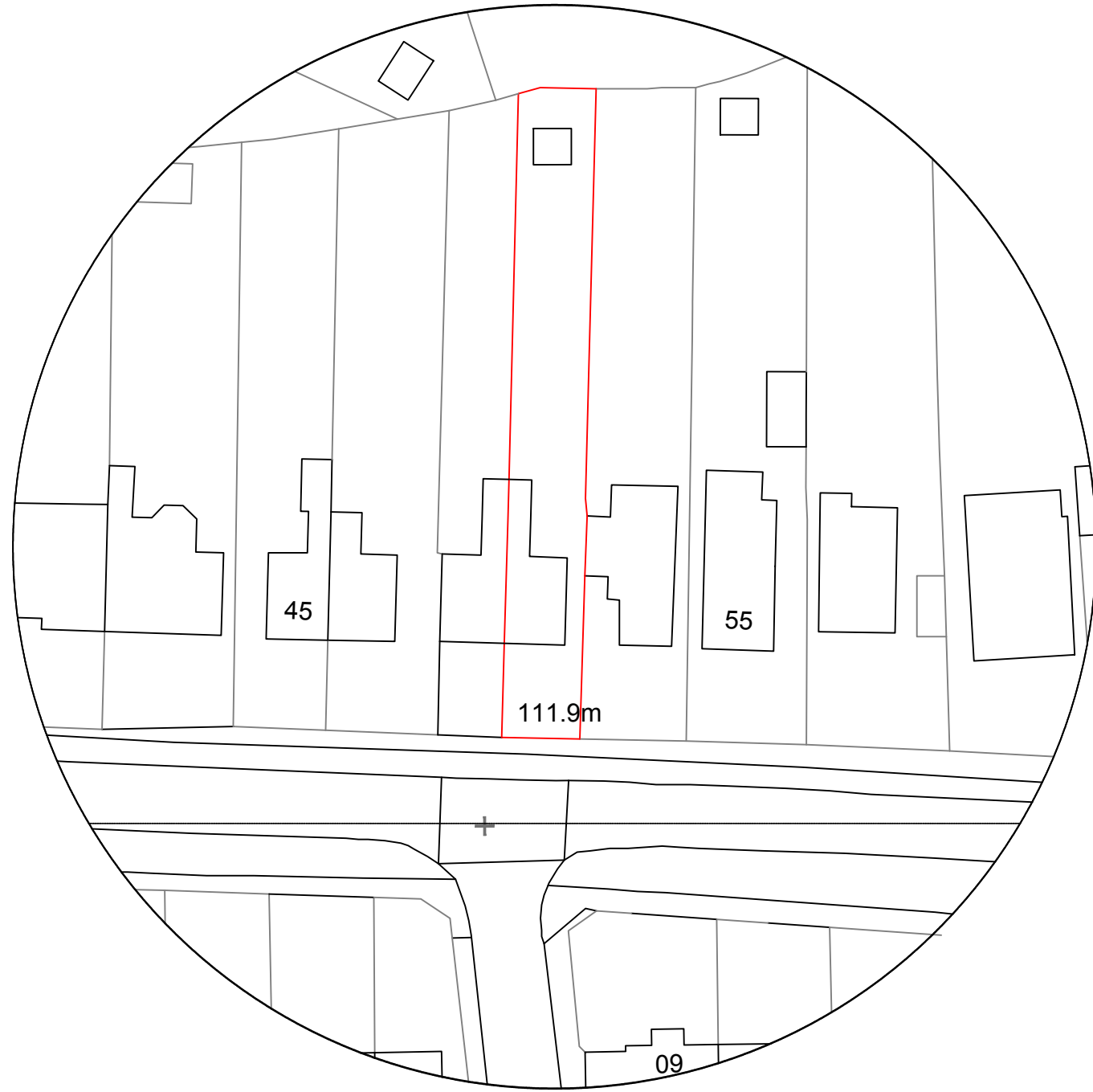
EXISTING SITE LAYOUT PLAN 1:500.
