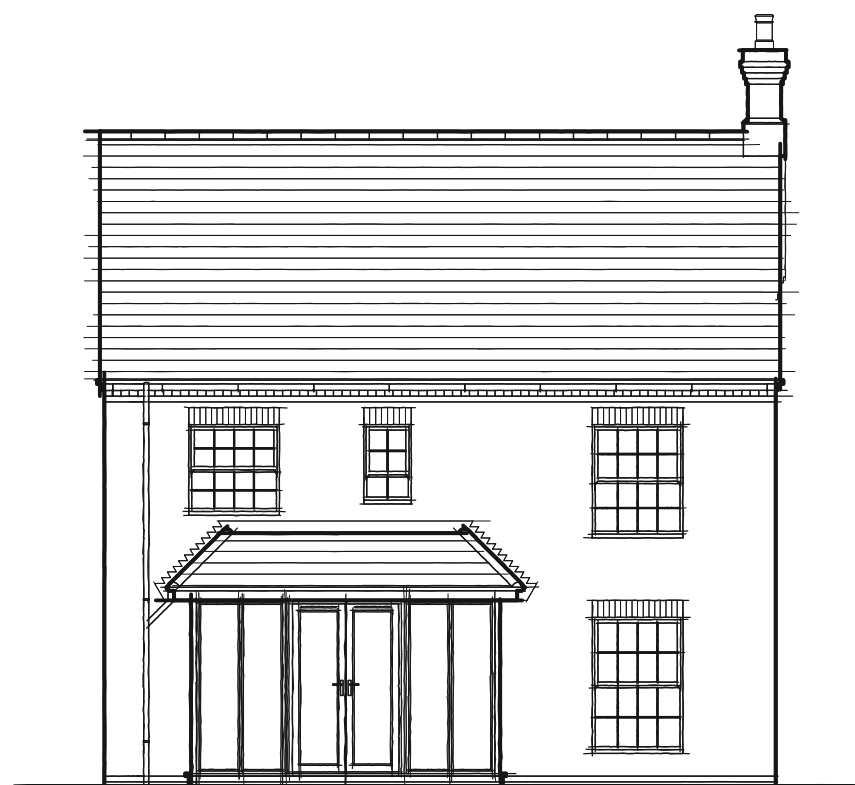
Rear Elevation
