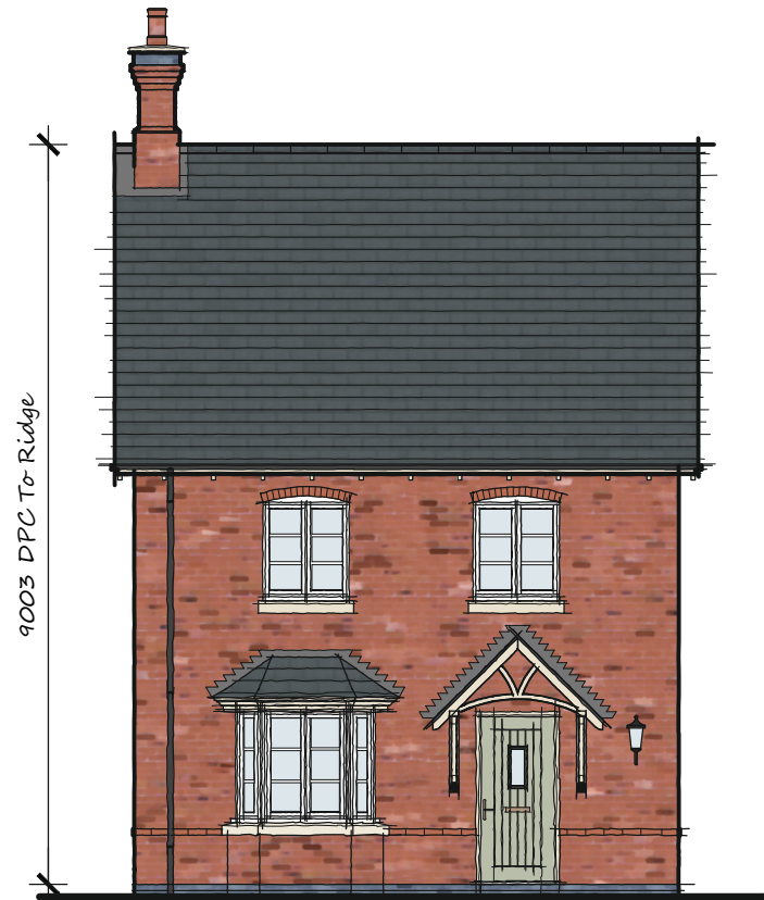
Front Elevation
