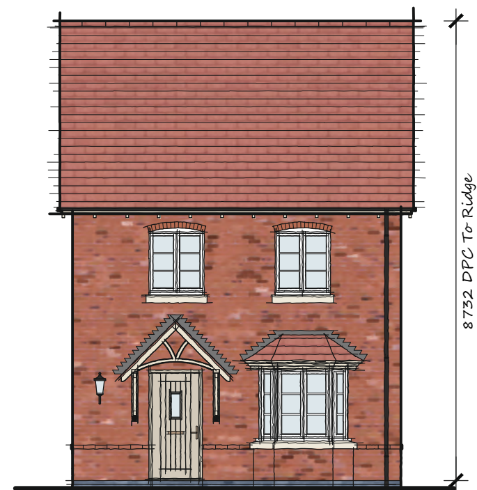
Front Elevation
