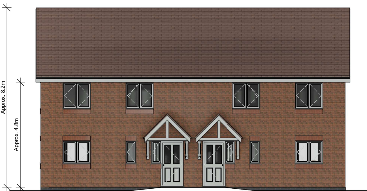
Front Elevation
