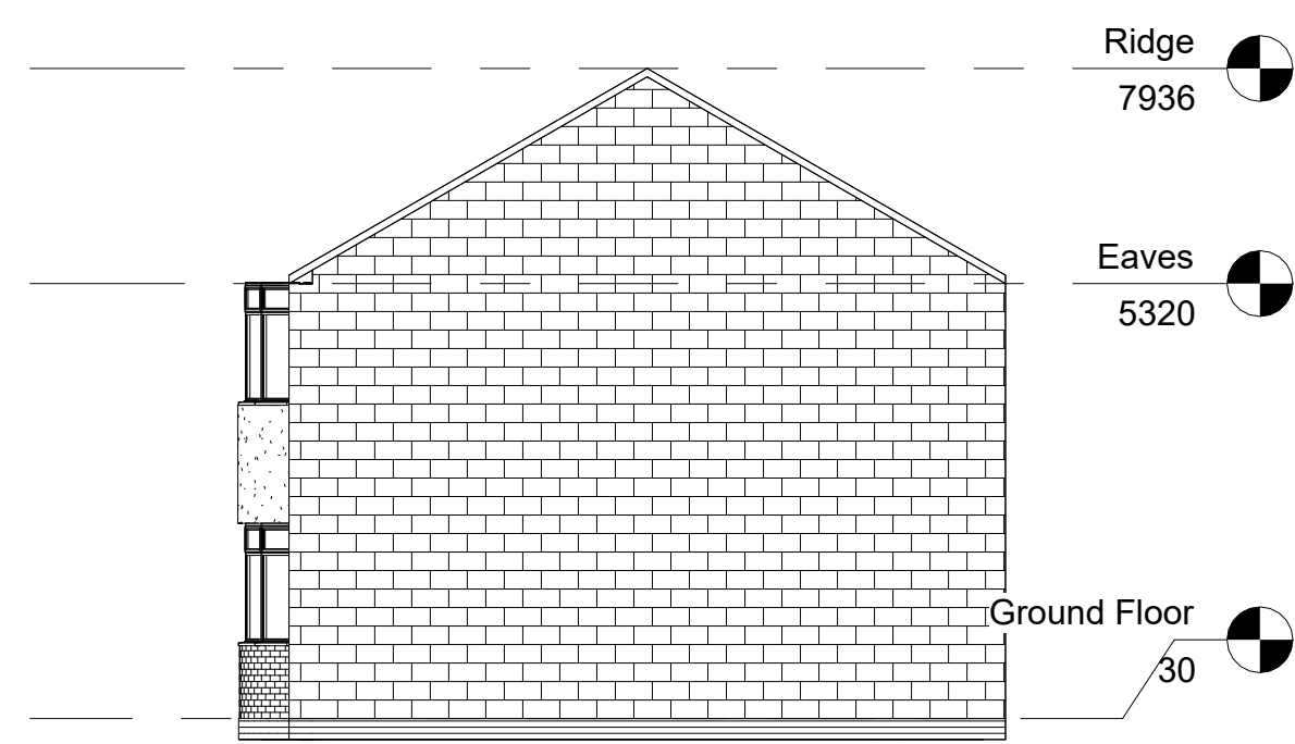
3 Proposed Side 1 Elevation 1 : 100
