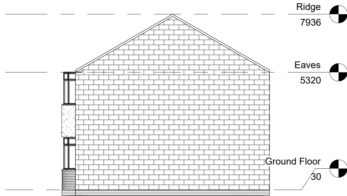
3 Existing Side 1 Elevation 1 : 100
