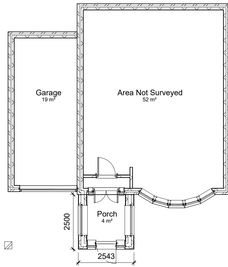
1 Proposed Ground Floor 1 : 100
