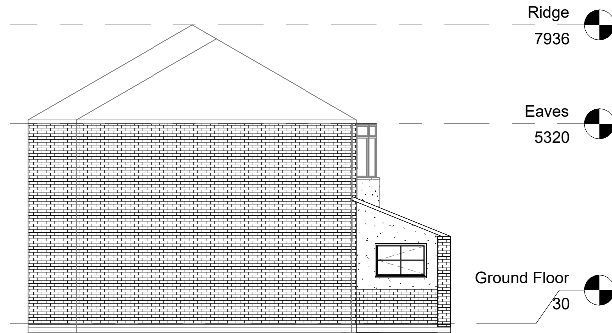
4 Existing Side 2 Elevation 1 : 100
