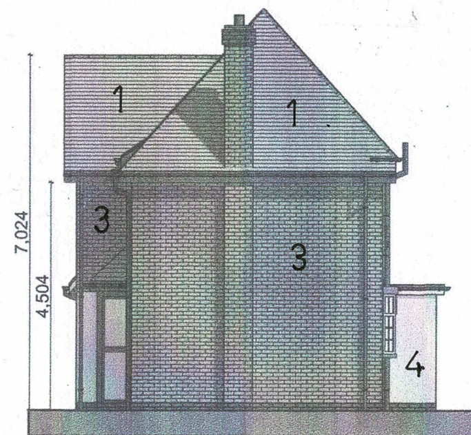
Side Elevation
